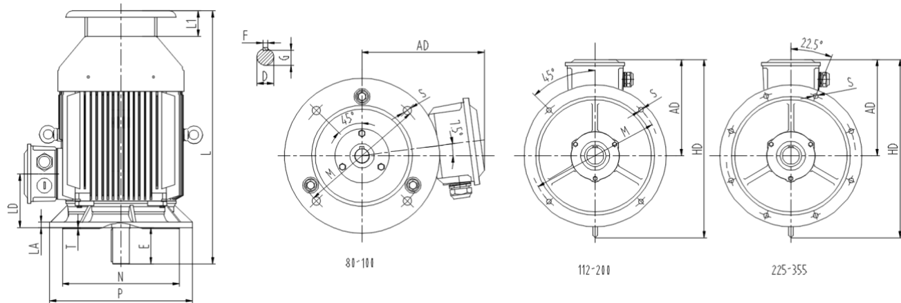
机械尺寸数据 (OMT4) Outline&Installation Dimensions (OMT4) V1
